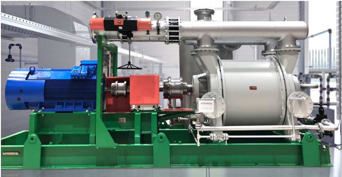
Single-stage Liquid Ring Package
